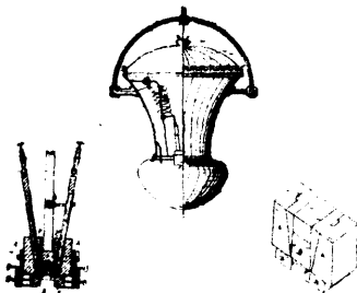
13351 Bureau's Improvements in Lamps.
