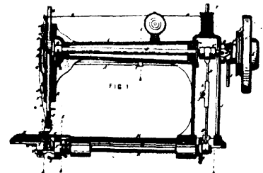
13350 Bond's Improvements on Sewing Machines.
