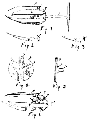
38525 Schellenberger's Earth Auger.
