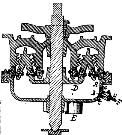
Reed's Bark Mills.
