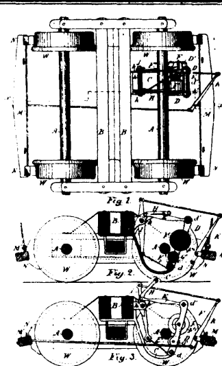
Hébert et al's, Car Brake.
