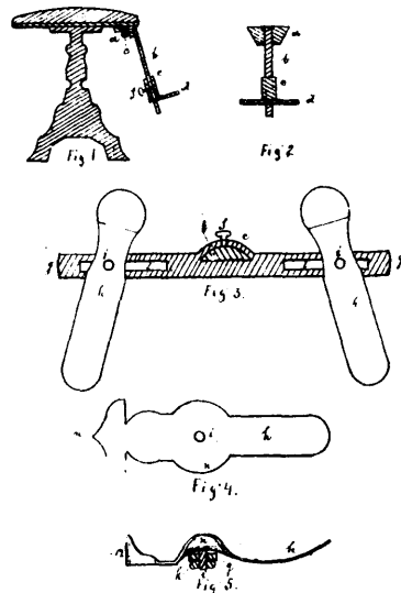
Burlingame's Foot Rest for Pianos.
