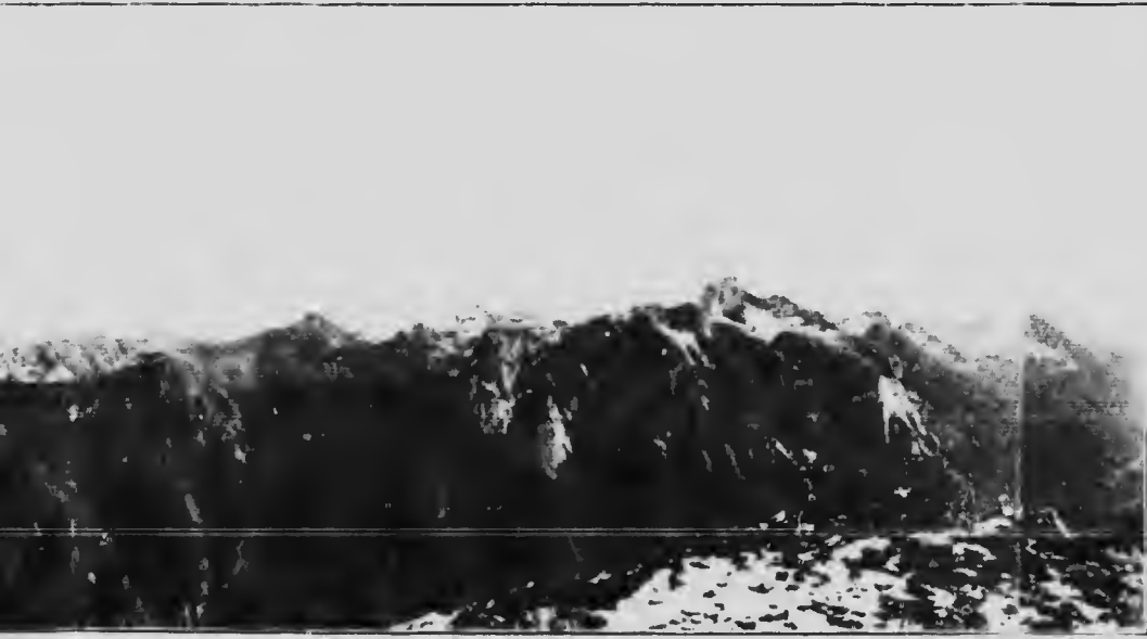
Black River valley on the left. View shows a concordance of summit levels.
