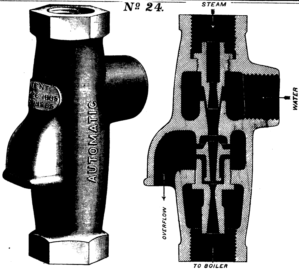
THE GRESHAM AUTOMATIC RE-STARTING INJECTOR.
