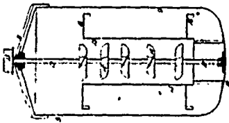
13666 Storer's Improvements on Process for Treating Liquids or Matters Dissolved or Suspended in Liquids, and in Effecting the Interaction thereof with Gases or Vapours for Promoting various Chemical and other Operations, and on Apparatus therefor.
