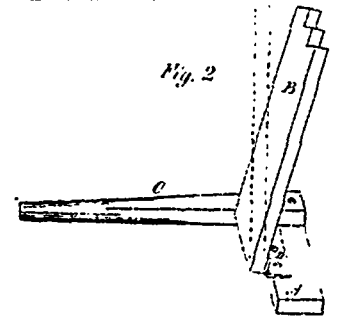
13686 Smyth's Improvement in Wagon Jacks.
