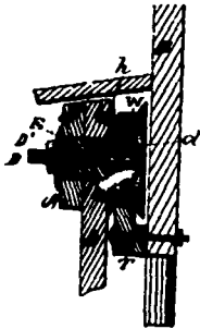
13674 Spiden's Improvements on Sliding Door Hangers.
