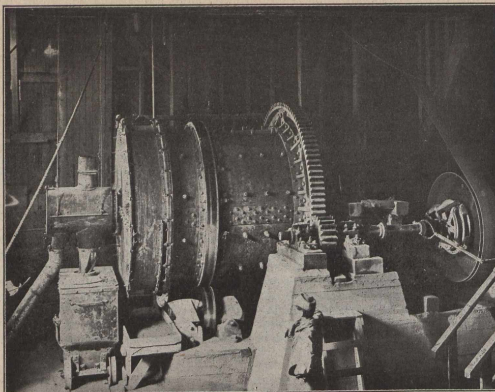
Ball Mill.
