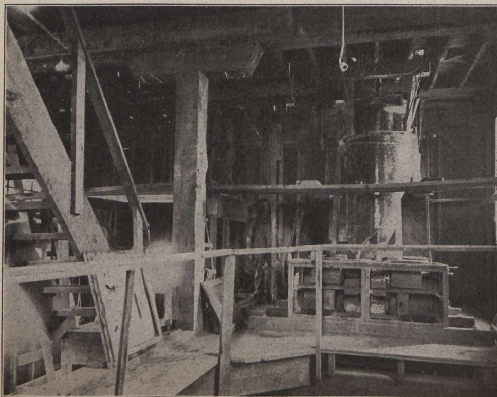
Spiral Mixer, Quartering Machine, and No. 1 Vezin Sampler.
