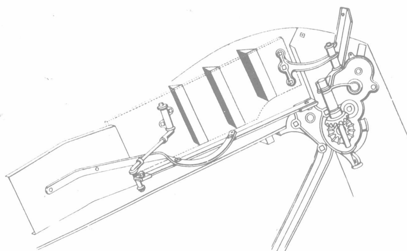
Butter Board on the Massey-Harris Light-Running No. 4 Binder.
