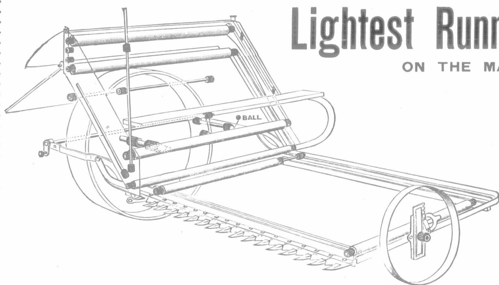
Roller Bearings wherever they will reduce friction.
