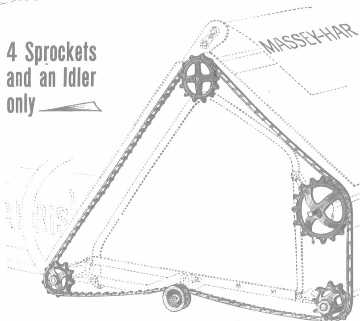
Chain Drive on Massey-Harris Light-Running No. 4 Binder.
