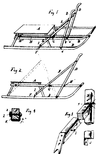
32569 Robbin's Sled Propeller.
