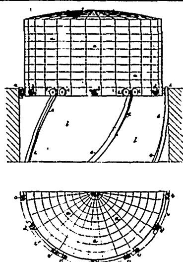
30001 Gadd's Improvements Relating to the Construction of Gas Holders.
