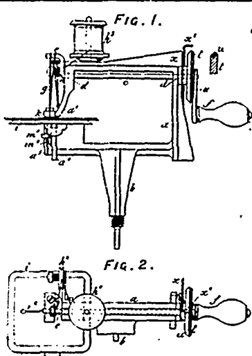
29000 Jackson &amp; Martin's Lock Stitch Sewing Machine.
