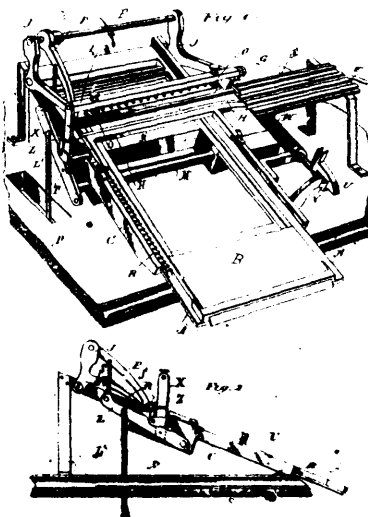
21554 Dement's Justifying Apparatus.
