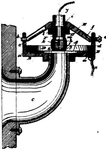
21549 Long's Telephone Transmitter.
