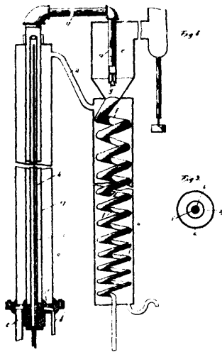
40740 Morrell's Apparatus for Evaporating and Concentrating Solutions.
