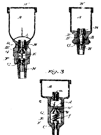
40745 Briggs' Lubricating Cup.
