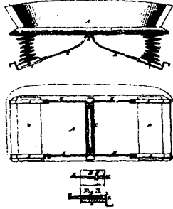
3415 Armstrong &amp; Armstrong's Spring Seat for Waggon and Cars.
