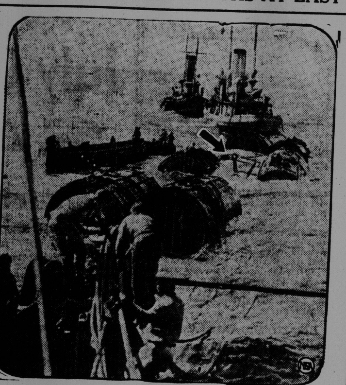
The U. S. submarine S-51, which sank off Block Island, R. I., in a collision 10 months ago, carrying all but three of her crew to death, is raised by the Navy salvage corps after months of effort and one earlier, fruitless trial. Photo shows the Falcon tugs, S-51, which is being hoisted from the water, indicated by arrow, can be seen between the forward pontoons.
