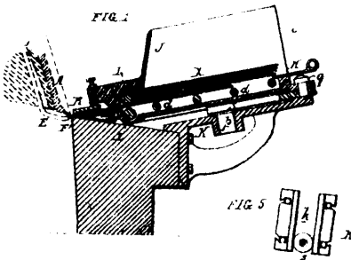
2162 Lawrence's Cut Nail Machine.
