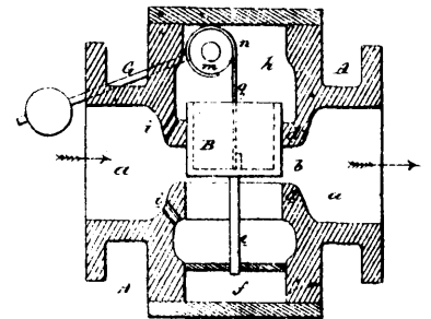
2164 Kitson &amp; Carr's Automatic Regulating Valve.
