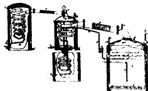
2166 Freatiss &amp; Howell's Apparatus for Distilling and Refining Petroleum, etc.
