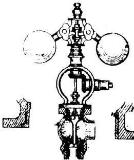
2159 Cogswell's Improvement on the "Judson Governor" for Steam Engines.
