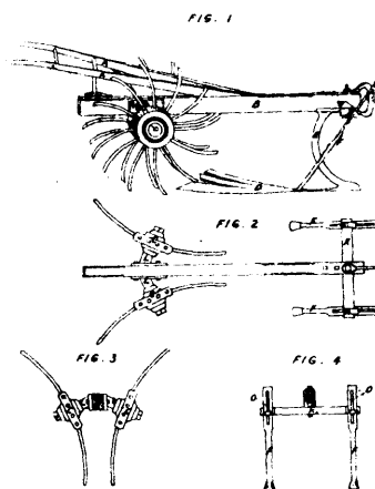
38699 Martin's Machine for Digging Potatoes.
