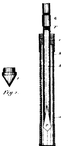
30586 Fontaine's Device for Boring Artesian Wells.
