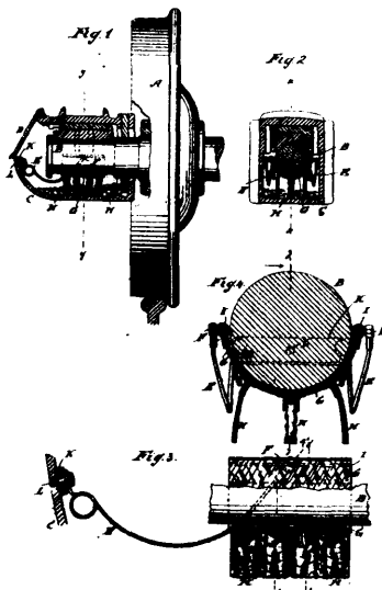
30592 Landau &amp; Scharfberg's Apparatus for Raising or Lifting Heavy Weights.
