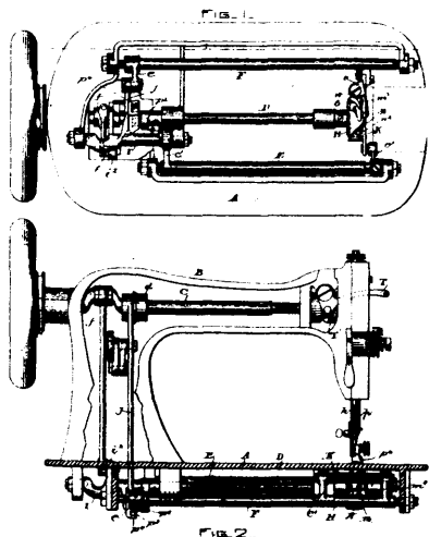
Diehl's Sewing Machine.
