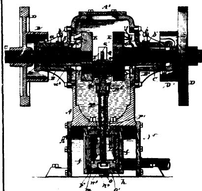
Case's Steam Engine.
