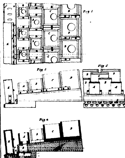
Hamilton's Reed Organ.
