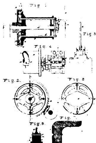
Flohr's Friction Clutch.
