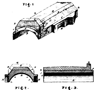
Kritch's Railway Car Axle Bearing.
