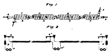
13034 Lugo's Improvements on Electric Circuits.
