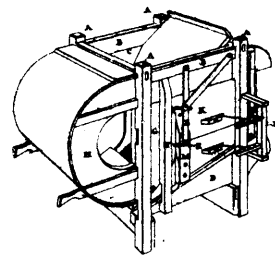
13039 Kline's Improvements on Fanning Mills.
