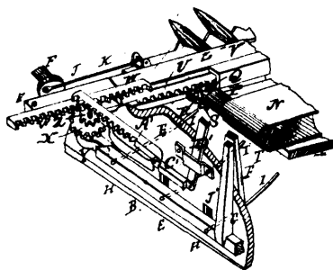
13033 Proper's Improvements on Combined Mowers and Reapers.
