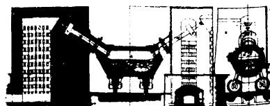
13045 Lindberg's Improvements in the Manufacture of Iron and Steel.
