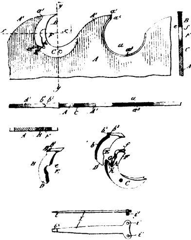
Brooke's Saw Teeth.
