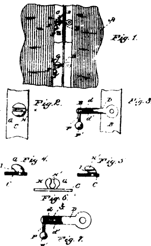
Bernstein's Fastening for Shoes, etc.
