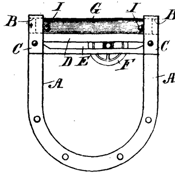
Moore's Door Hanger.
