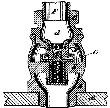
37473 Hanna's Process of and Apparatus for Purifying Water.
