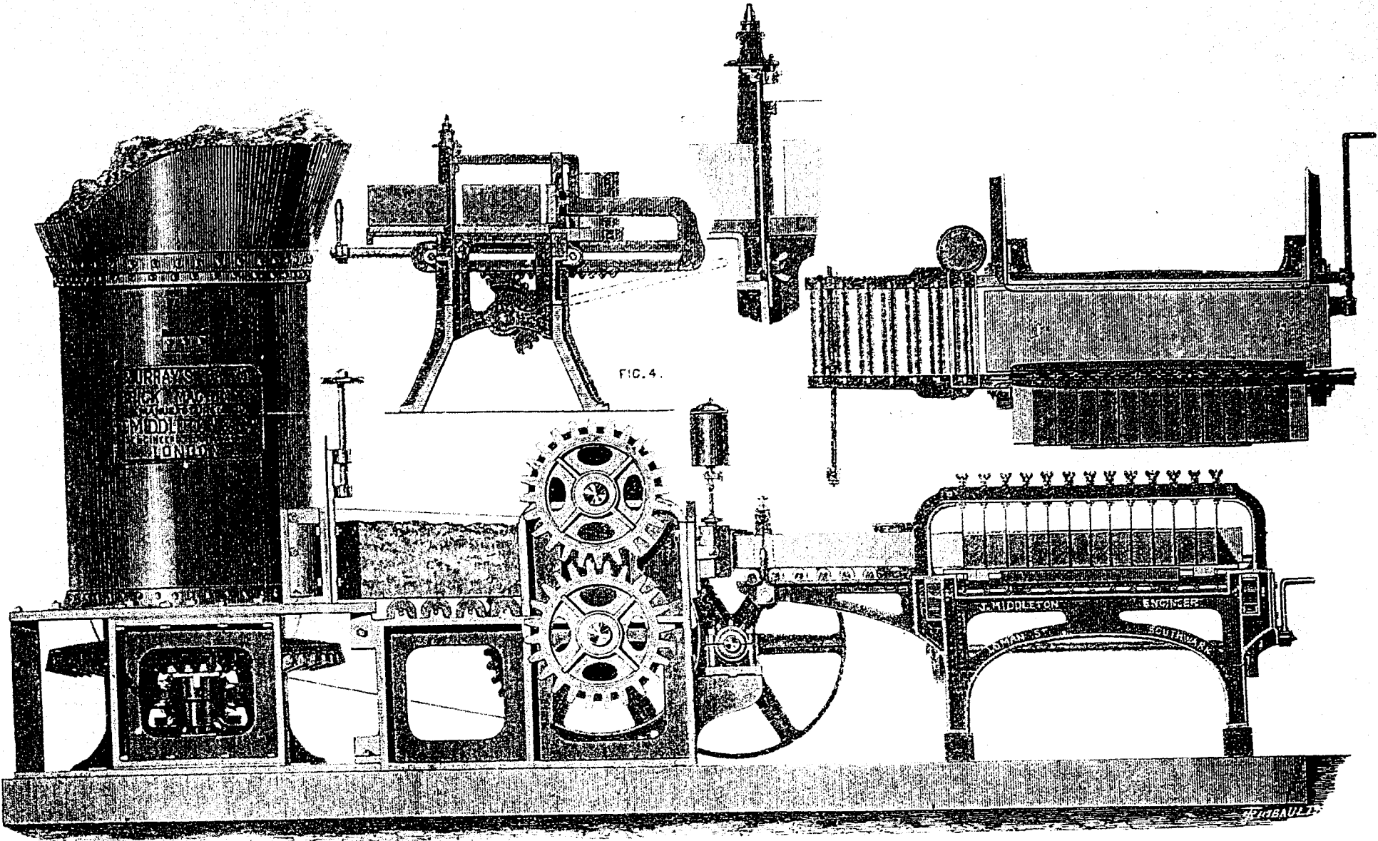
MURRAY'S CONTINUOUS DELIVERY BRICK-MAKING MACHINE
