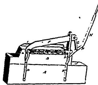
8089 Broderick &amp; Cook's Machine for Cutting Iron and other Metals.
