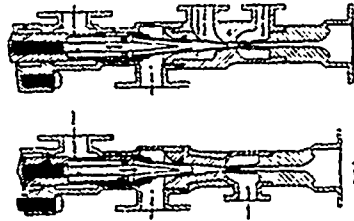
8086 Hamer, Metcalfe, &amp; Davies' Improvements on Steam Boilers.
