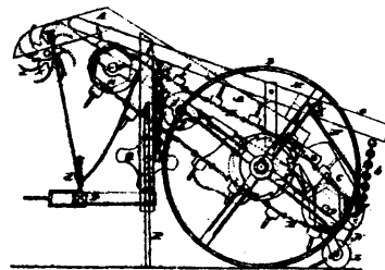
4436 Young's Hay-loader.
