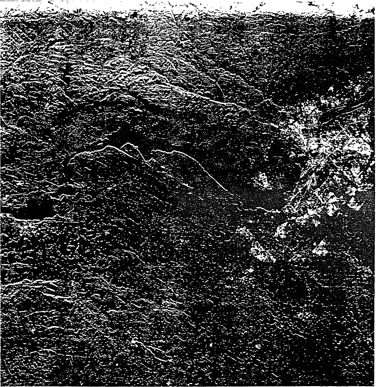
Figure 10: Wide Swath Image of the Outaouais Region.
