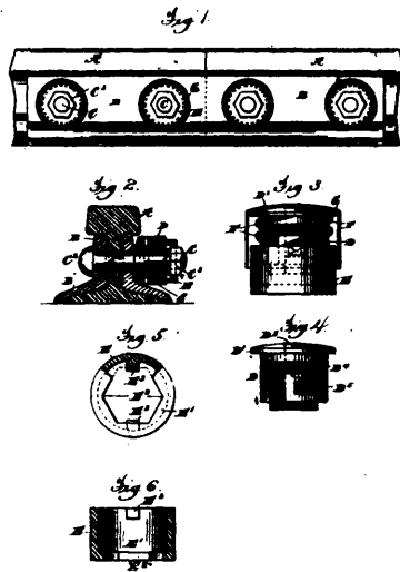
26304 Bessel's Nut Lock.
