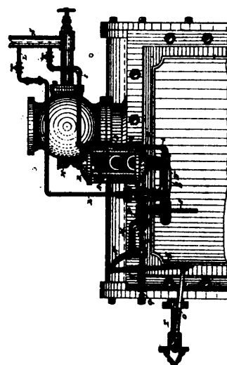
17386 Jareochi's Lubricator for Cylinders of Steam Engines.
