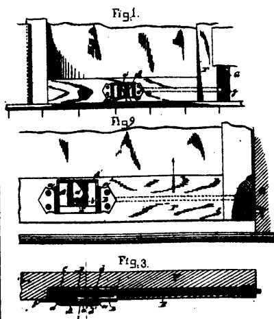
17387 Elliott's Improvements in Sash Lifters and Fasteners.
