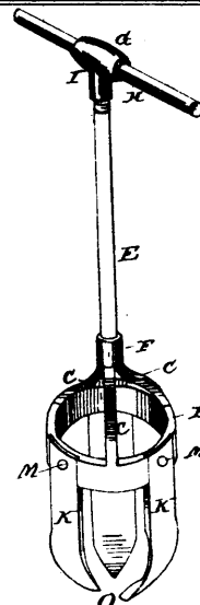
17383 Switzer's Improvements in Post-Hole Diggers.
