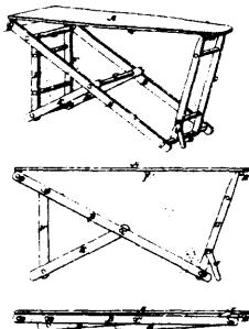
3040 Scofield &amp; Wait's Ironing Table.
