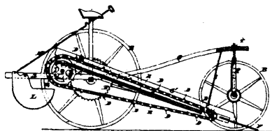
3038 McCallum's Potato Digger.
