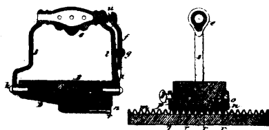
3042 Hewitt's Smoothing, Band, Glossing and Fluting Iron.
