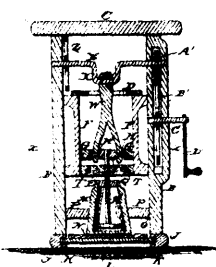
13499 Flood's Improvements on Churn Motors.
