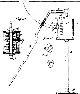
13502 Howard's Improvements on Draughting Instruments.
