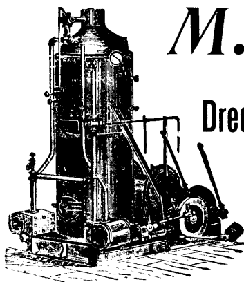
UNION GAS OR OIL ENGINE & HOIST COMBINED—On Strong Iron Base. 6 to 50 h.p. of design shown in cut.
