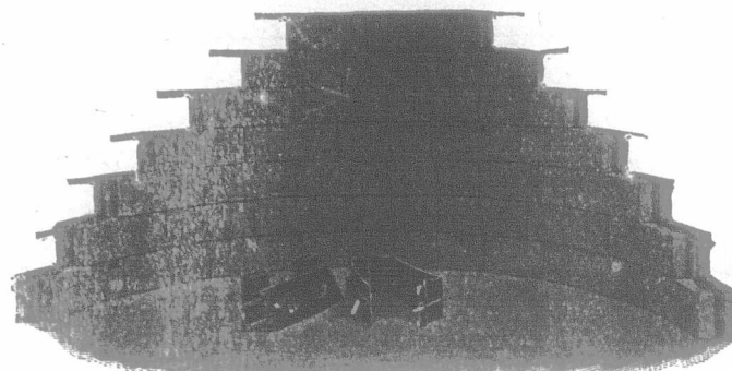
Section of Wall Laid up with Interlocking Continuous Air Space Concrete Blocks
