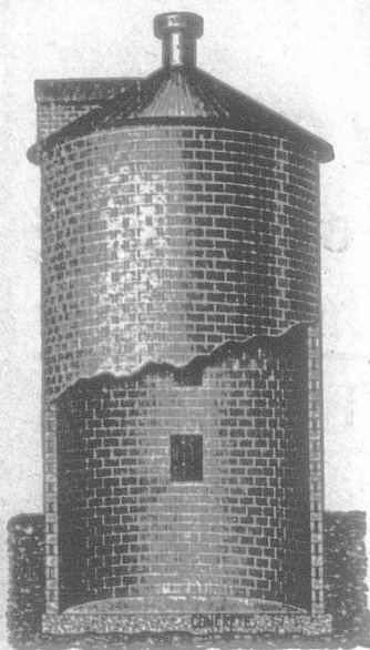
Section of Silo Built from Interlocking Continuous Air Space Concrete Blocks
