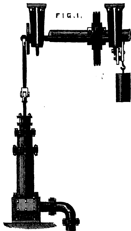
FRICTION GEAR FOR DRIVING PUMPS.
