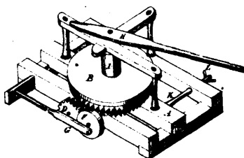
6337 Gibson's Improvements on Horse-powers.
