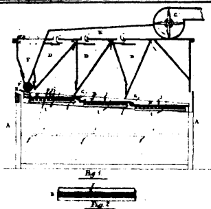
6325 Barter's Middlings Purifying Machine.
