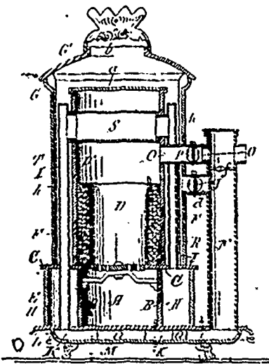
25369 Van Wormer's Heating Stove.
