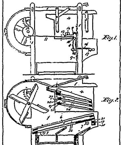
25371 Jackson's Panning Mill.
