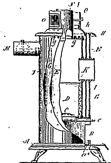
25367 Van Wormer's Heating Stove.
