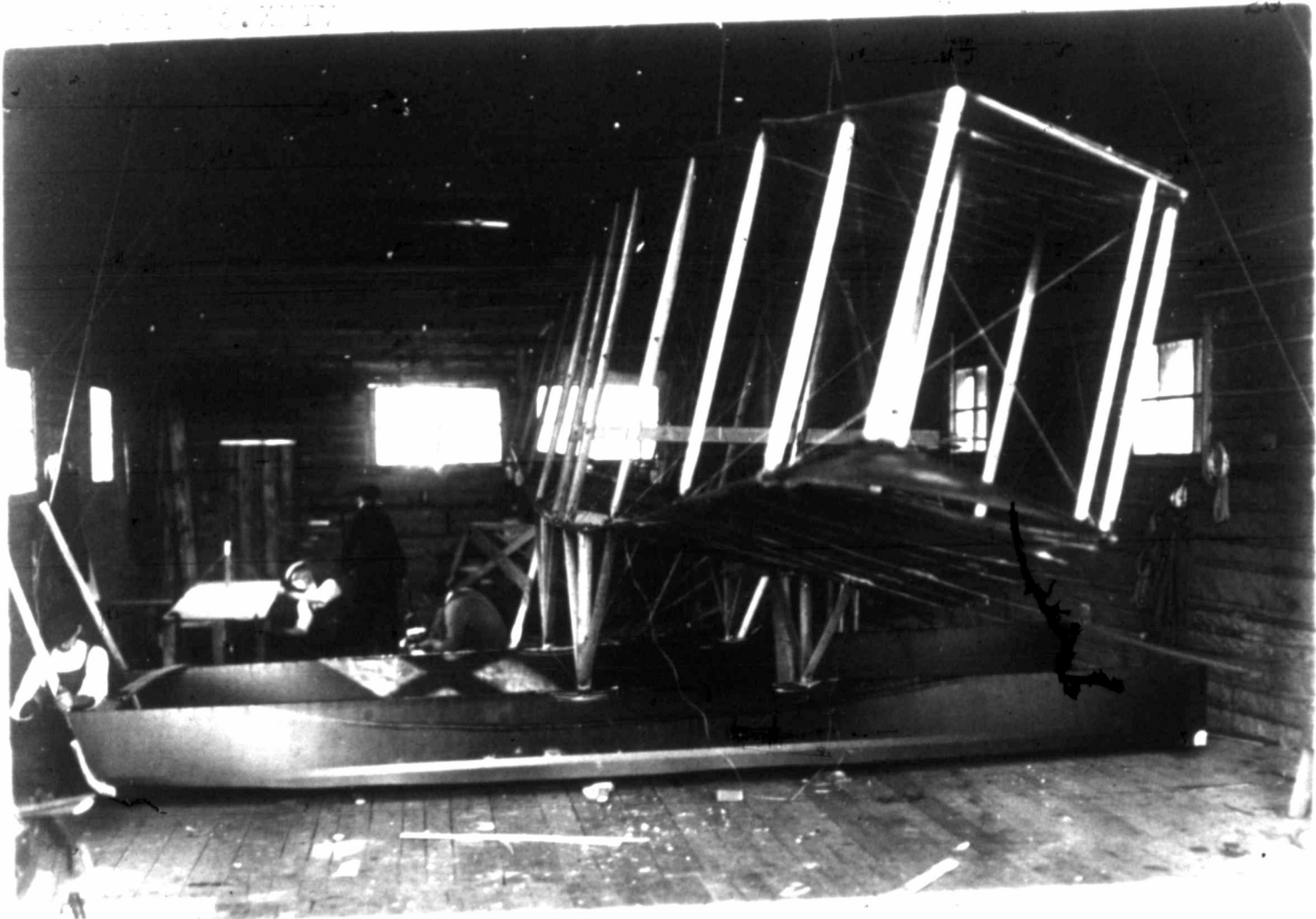
First view of the hull
