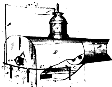
14252 Orvis's Improvements on Steam Boiler Furnaces.
