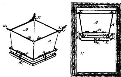
14248 Gurney's Improvements on Refrigerators.
