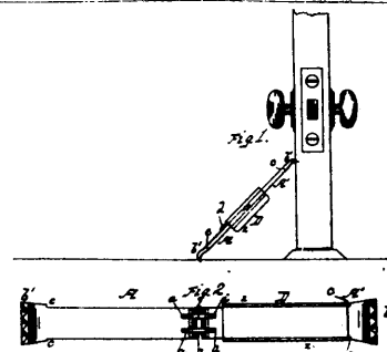
14257 Lockwood's Improvement in Door Securers.
