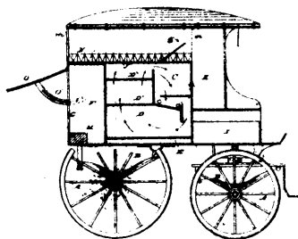
14249 Gurney's Improvements on Refrigerator Waggon.
