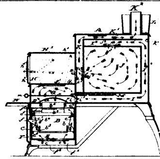
14245 Vining & Quesnel's Improvements on Cooking Stoves.
