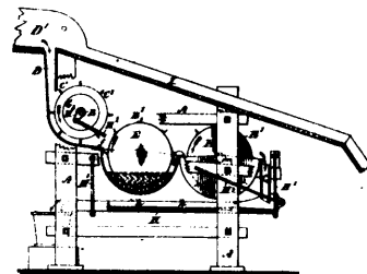
14251 Taylor's Improvements in Apparatus for Separating and Amalgamating Gold and other Precious Metals.
