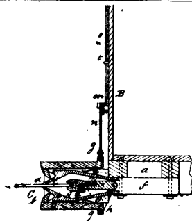
14256 Chase's Improvement in Car-couplings.
