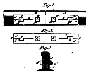
14254 Macdonald's Improvement on Nut Locks.
