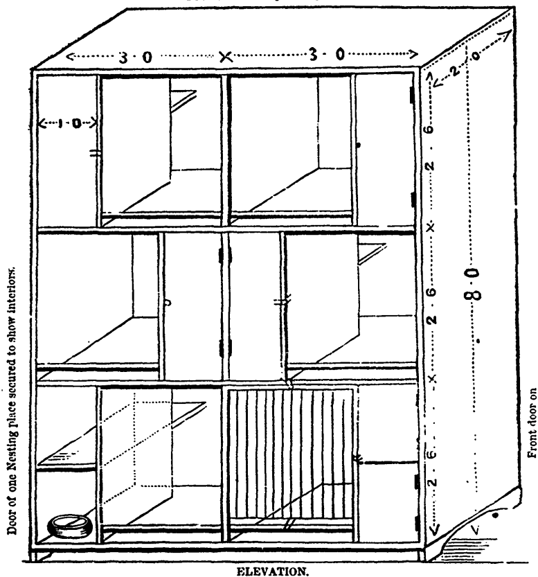
PIGEON BOX— \frac{1}{2} -inch by 1 foot.
