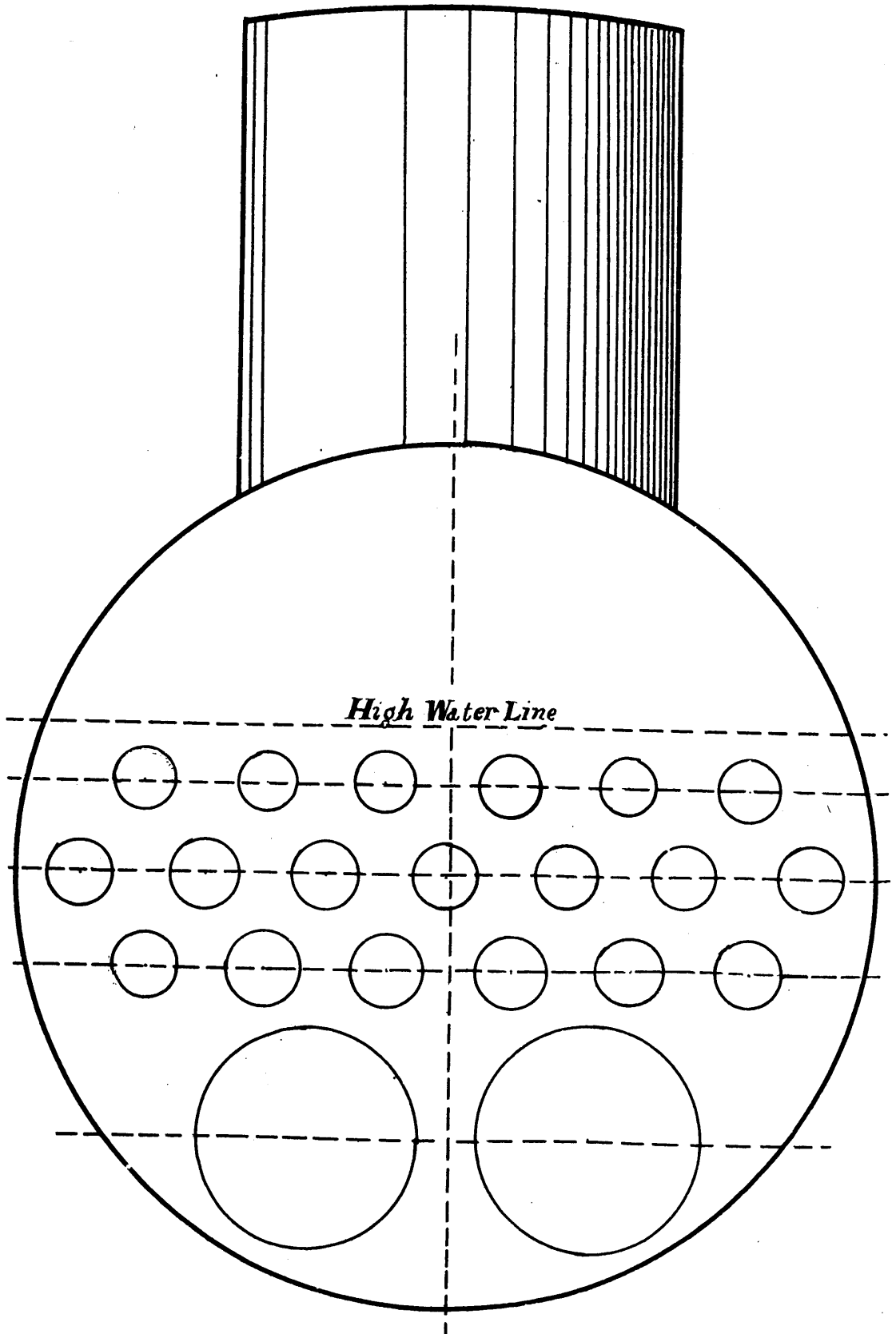
A CHAPTER ON BOILERS.—BY P. S. OF TORONTO. (See description page 221.)
