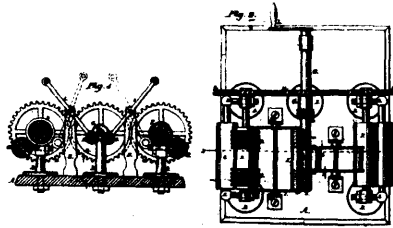
4838 Kitzmiller & Smith's Broom Handle Painting Machine.
