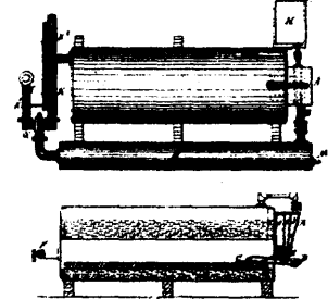
4843 Ramsden's Method of and Apparatus for Securing the Combustion of Fuel and for the Utilization of Gases thereof.
