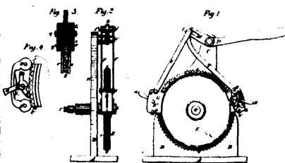
4847 Bond & Shoff's Pawl and Ratchet Mechanism.
