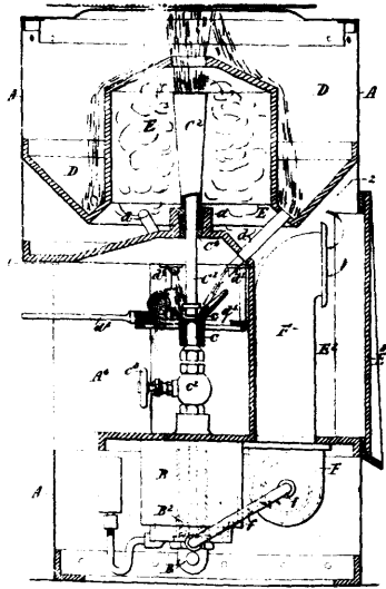
Mathewson's Sand Blast Apparatus.
