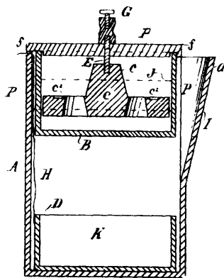
Thurber's Wind Mill.
