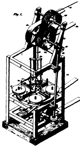
83224 Beale's Machine for Winding Wire with Covering Material.
