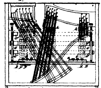
83232 Richards' Shifting Piano Action.
