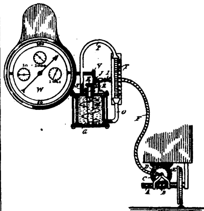
19646 Cowell's Speed Gauge for Locomotives.
