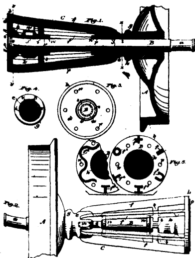
19648 Eaton's Car Axle Truss.
