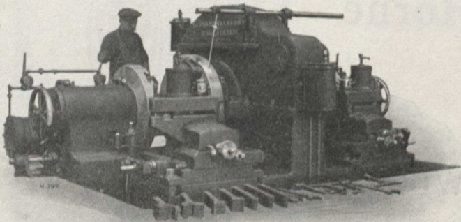
80-Inch 'Double' Driving Wheel Lathe--Motor Driven.
