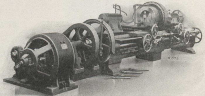
Double Car Axle Lathe.
