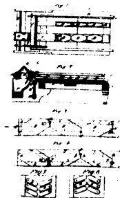
9299 Bacon's Improvements in Ink Distributing Apparatus.
