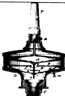
9300 Thompson, Whaley &amp; Cohen's Improvements in Gas Controllers.
