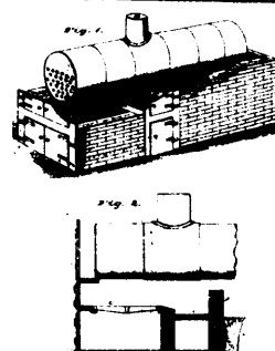
9298 Fisher's Improvements on Boiler Furnaces.
