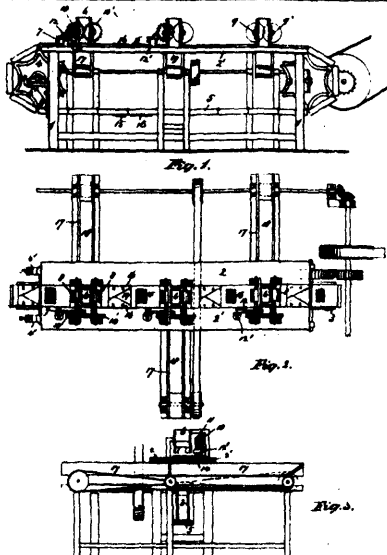
18184 Millen &amp; Mousseau's Match Splint Machine.
