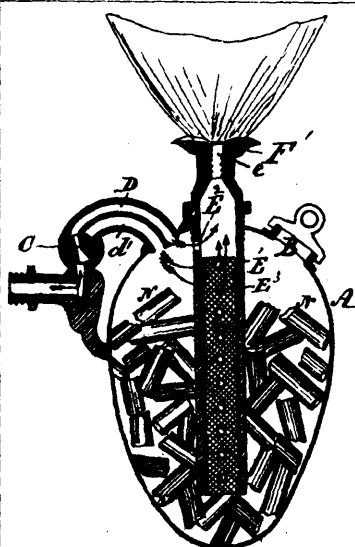
18182 Livesey &amp; Kidd's Apparatus for Enriching Illuminating Gas.
