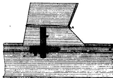
10190 Crabb's Method of Fastening Carriage Seats.
