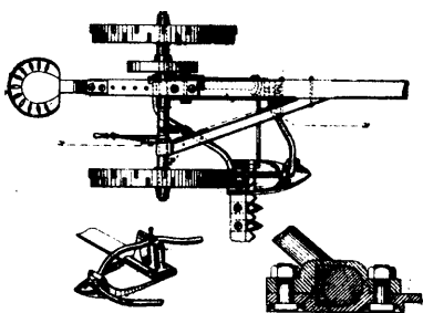
10185 Manny's Improvements on Harvesting Machines.
