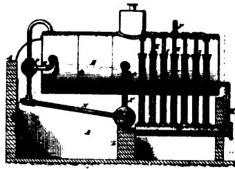
7530 Smith's Improvements in Furnaces for Steam Boilers.
