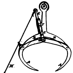
7544 Ella's Improvements on Horse Hay Forks.
