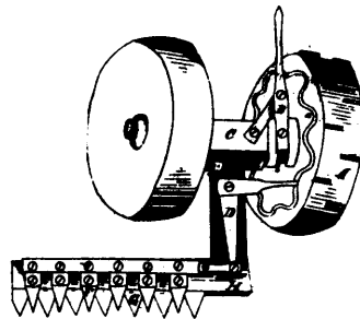
7539 Jones' Improvements in Mowers and Reapers.
