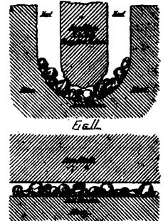
7537 Tilghman's Improvements on Sawing Stones.
