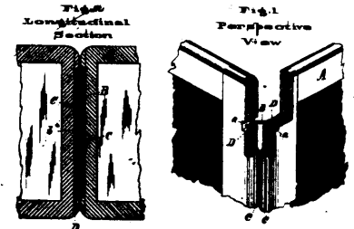
7534 Van Kannel & Rapp's Reversible Hinged Slates.
