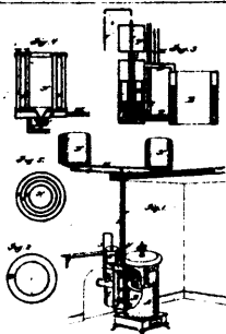
5171 Richardson's Steam Heating Apparatus.
