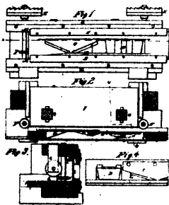
5170 Skidmore &amp; Moore's Hoop Machine.
