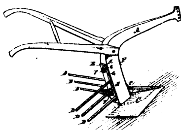
5178 Bolton's Potato-digger.
