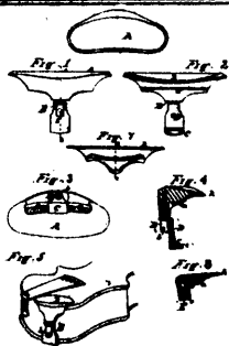
5166 White's Chin-Res for Violins.
