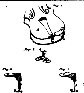
5167 White's Chin-Res for Violins.
