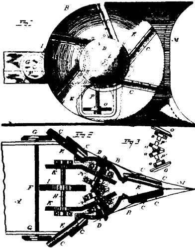
22269 Morgan's Rotary Snow Plough.
