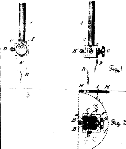
22276 Eastwood's Attachment for Sewing Machines.
