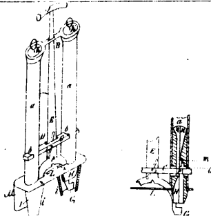
6065 Carr's Improvements on Seed Planters.
