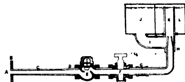
6063 Howell's Machine for Heating Locomotive Water.
